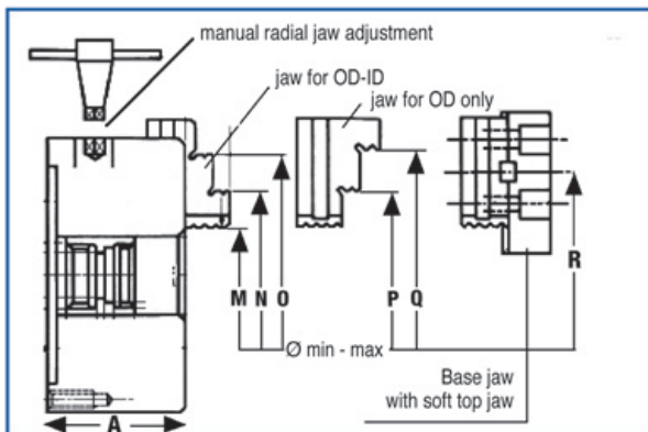
Pneumatic or hydraulic rotating cylinder power clamping 3 mm. stroke for each jaw
