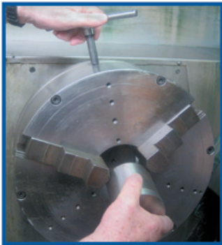
Continuous manual jaw radial adjusting by means of key
